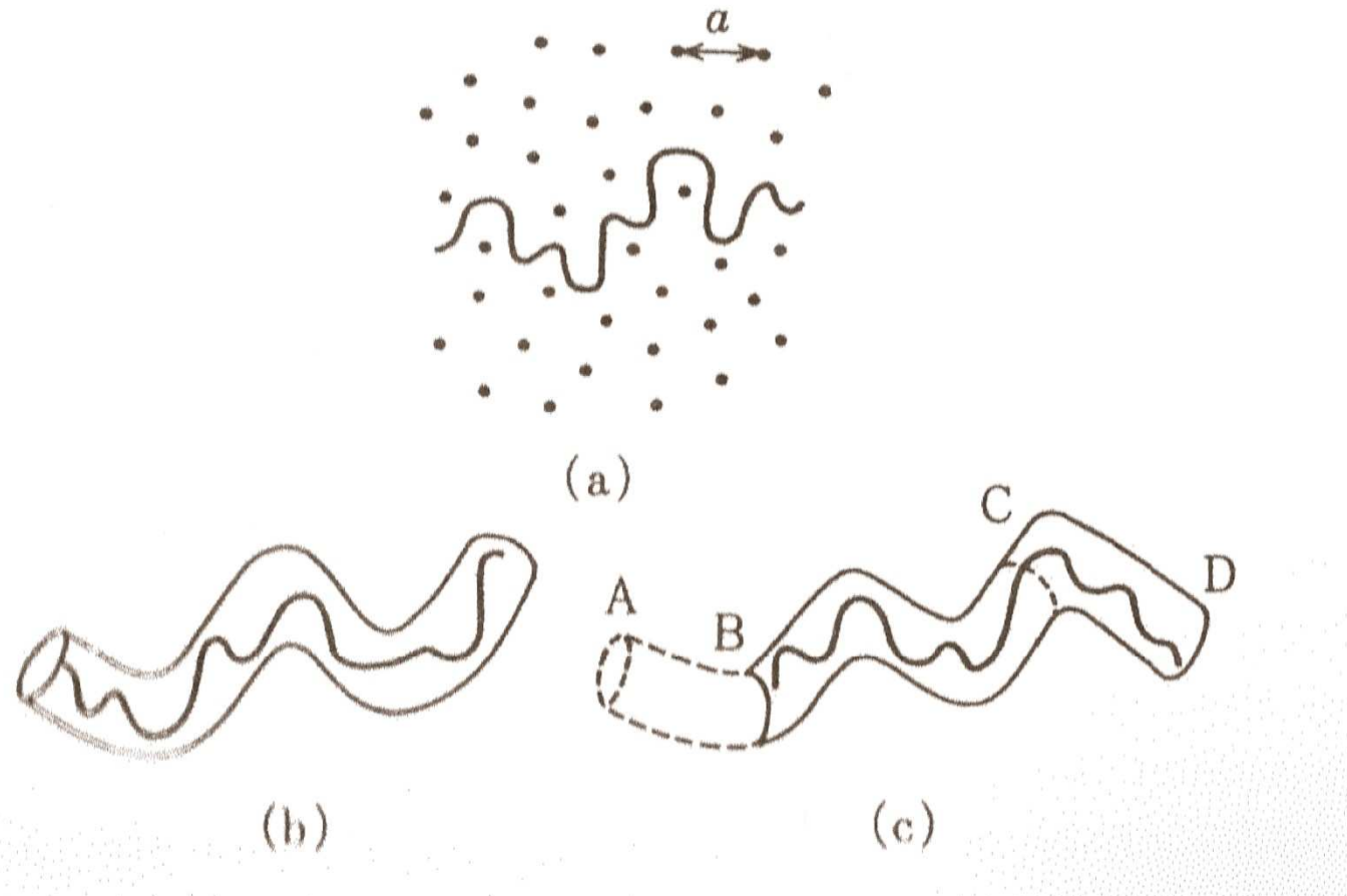
(a) A polymer moving in a fixed network; (b) the tube model; (c) the situation depicted in (b) after some time has passed
