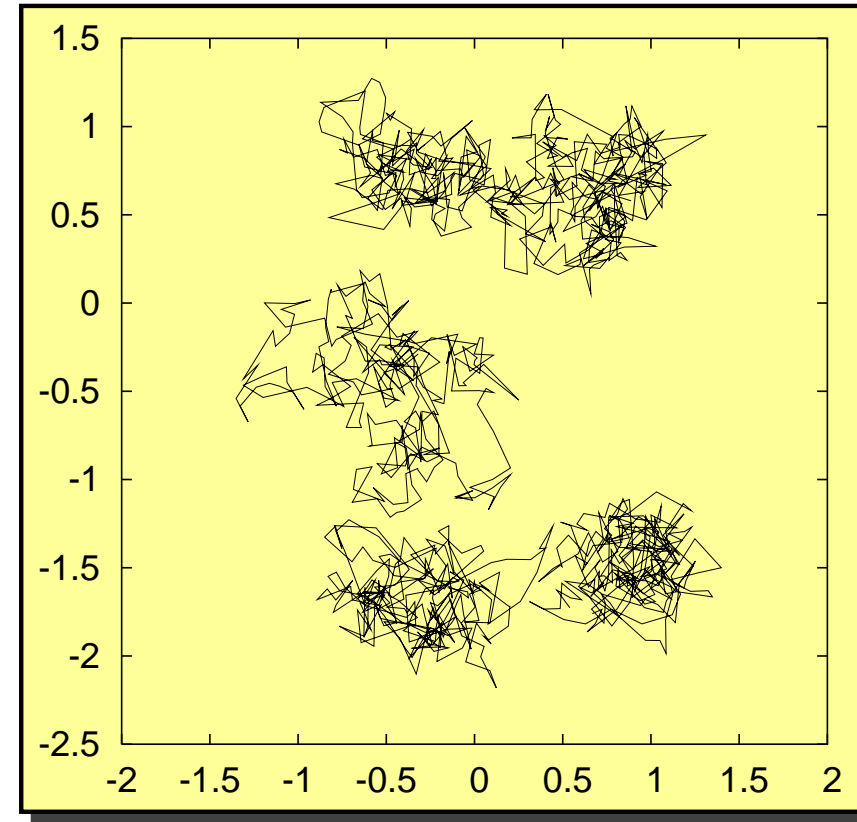
5 H 2 molecules with 256 beads at T = 1 K
