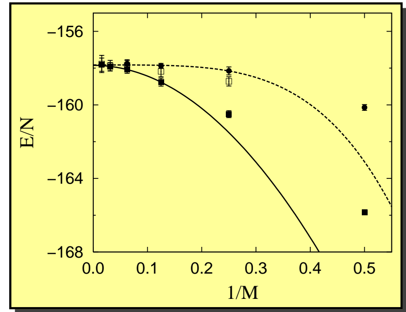
Liquid Ne, \rho = 0.0363 \text{ \AA}^{-3}
