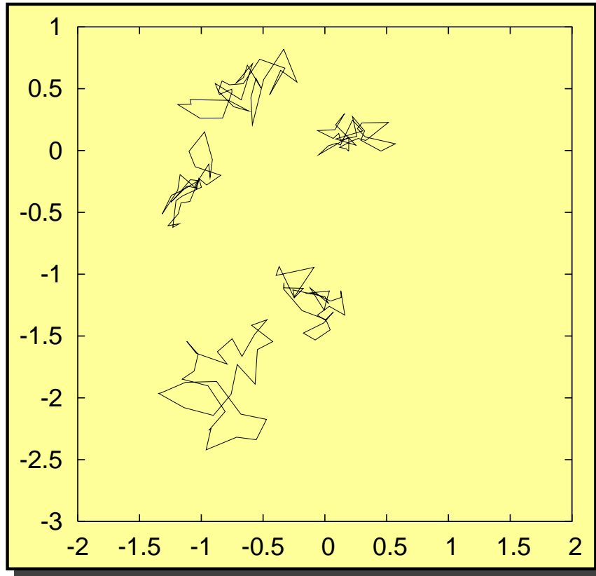
5 H 2 molecules with 32 beads at T = 6 K
