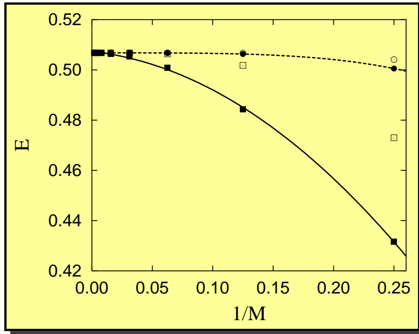
1D Harmonic oscillator
